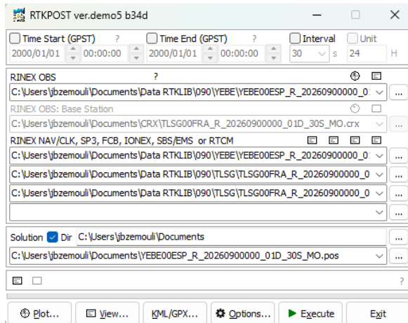
(a) Interface principale de RTKPOST.
