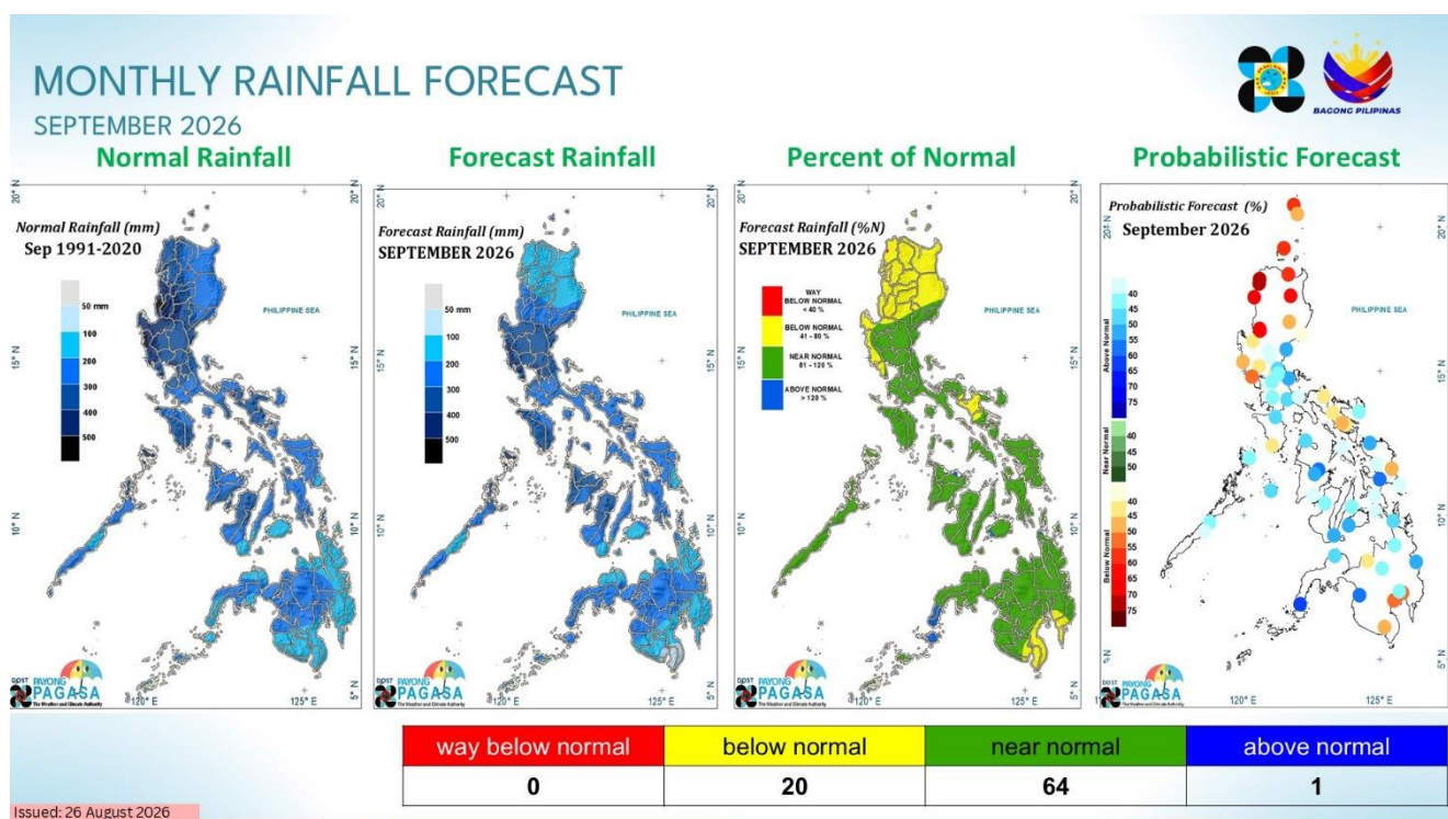
Figure 2: Monthly Rainfall Forecast for September 2026
