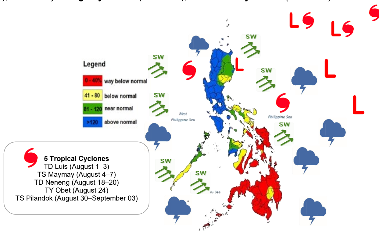
Figure 1: Actual Rainfall and weather systems experienced for August 2026
