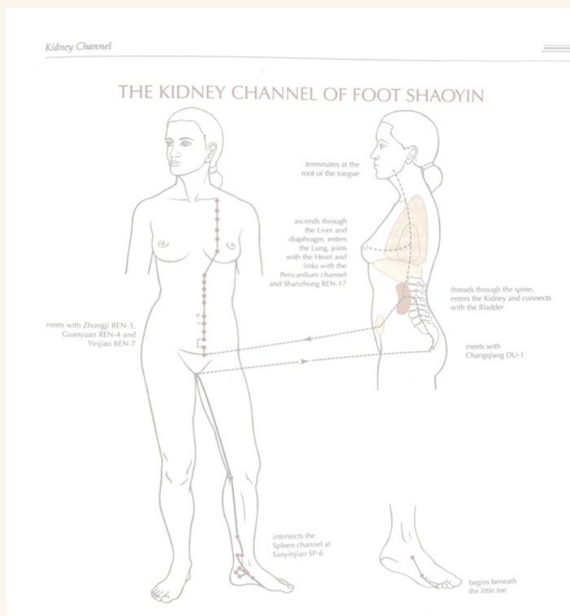
Col. Fig. 9 The Kidney Meridian of Foot Shaoyin
