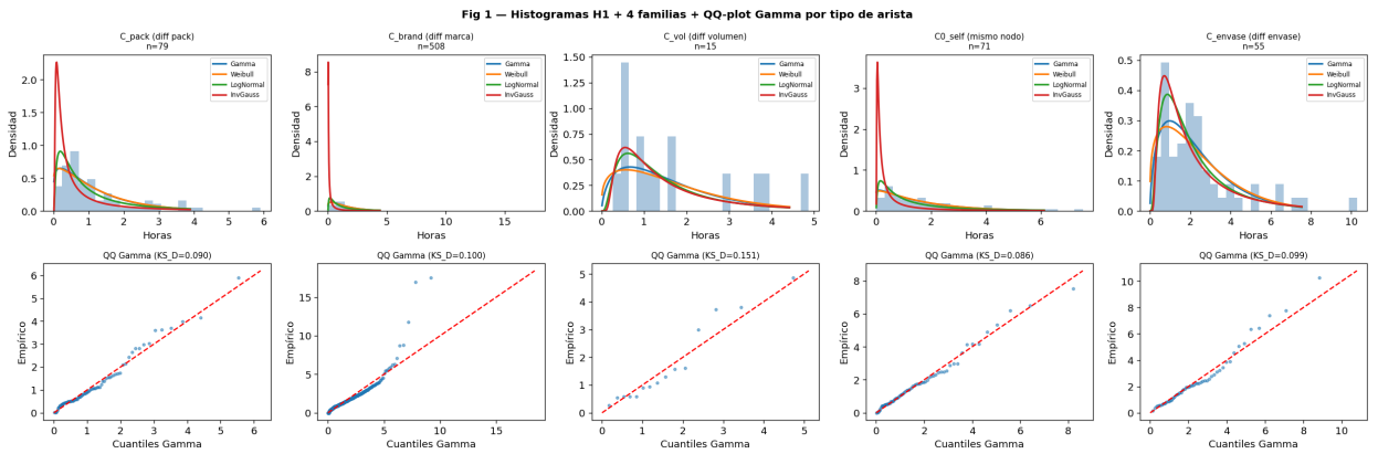
Figure 3: Per-type histograms on H_1 with the four fitted densities (top) and Gamma QQ-plots (bottom). Points on the diagonal indicate an adequate fit; the heavier upper tail of C\_envase is apparent.
