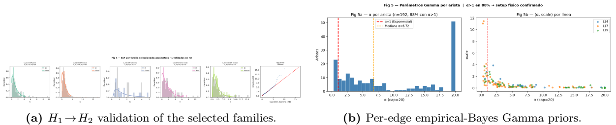
Figure 6: Out-of-sample fit and hierarchical priors. Left: the family chosen on H_1 still describes H_2 for the stationary types. Right: distribution of the per-edge shape parameters; most edges fall back to the global prior.
