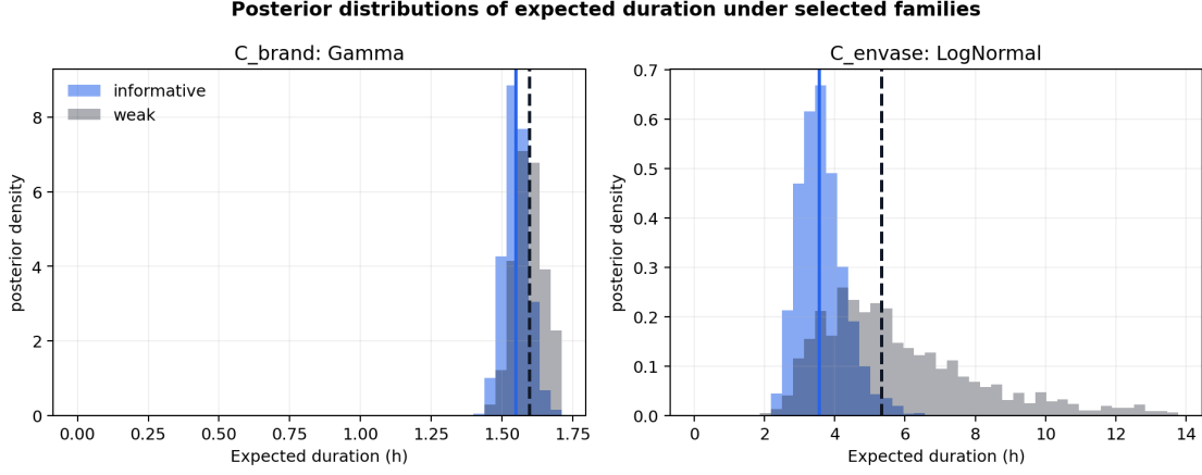
Figure 5: Posterior densities of the expected duration for a data-rich type (C_brand) and a long-tailed type (C_envase). The LogNormal posterior for C_envase explicitly carries the risk of long label-reference changes.
