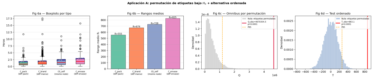
Figure 7: Application A (edge types). From left: boxplots, mean ranks, omnibus null distribution of Q , and null distribution of the ordered statistic T . The observed statistics lie far in the right tail of their permutation nulls.
