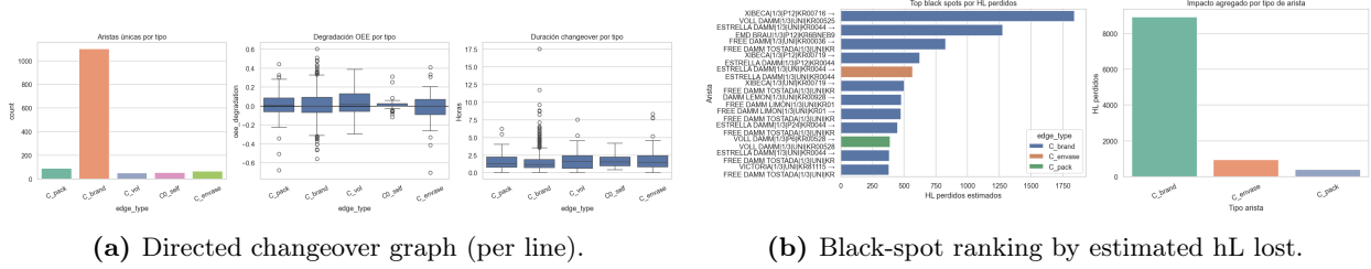
Figure 10: Post-mortem of the 2025 history: the directed transition graph and the ranked black spots that drive avoidable loss.
