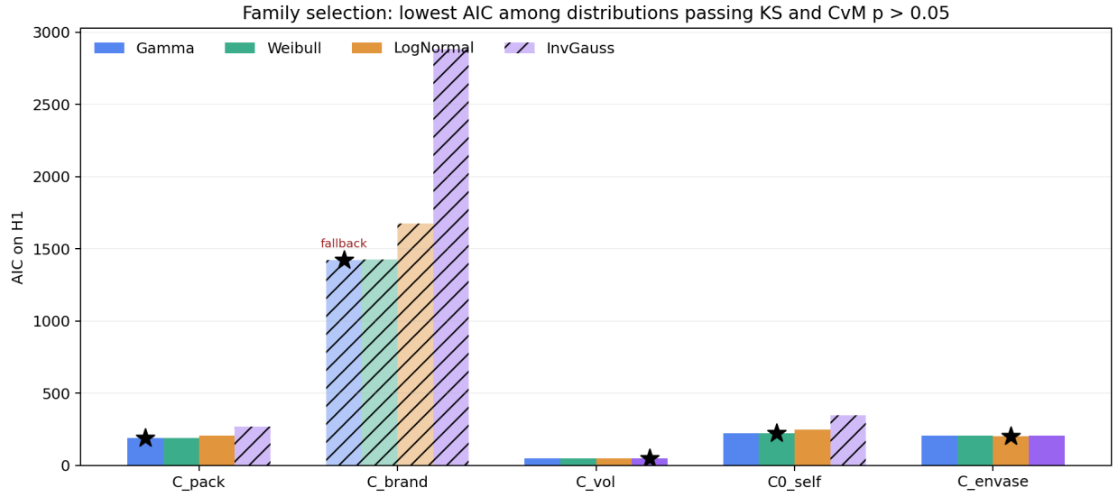
Figure 2: Family selection by edge type. Solid bars pass both KS and CvM diagnostics; hatched bars fail at least one diagnostic. The black star marks the selected family.
