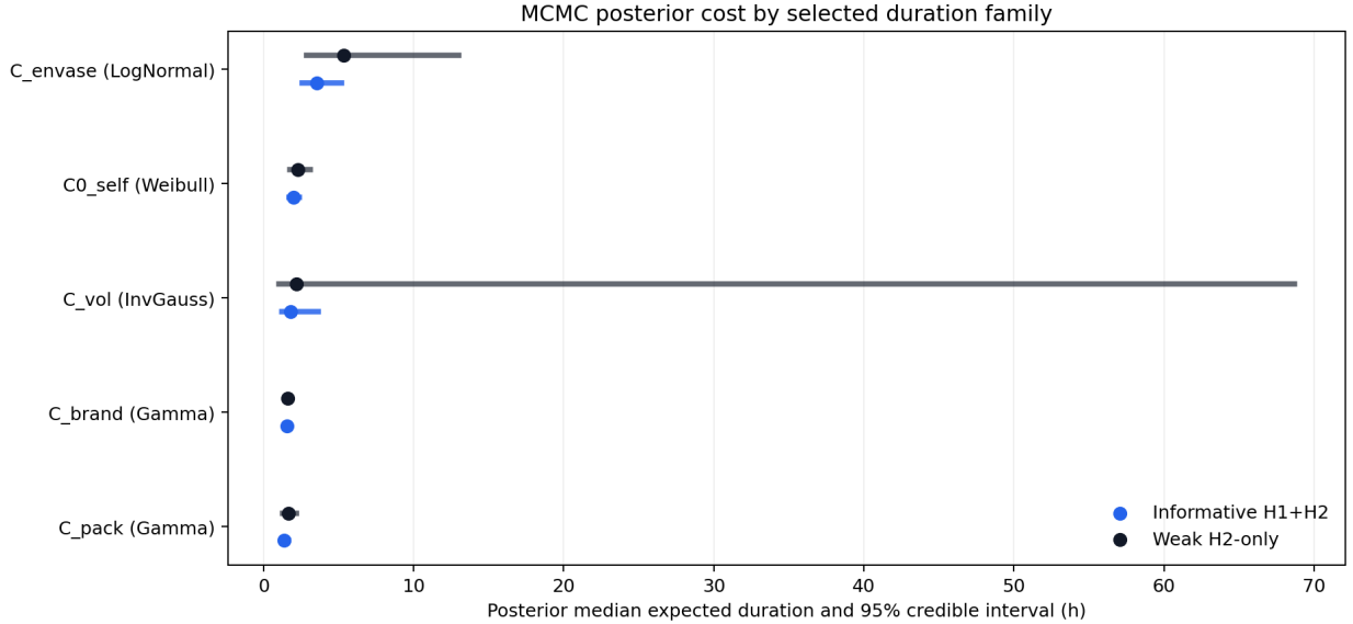
Figure 4: Posterior expected duration by selected family. Blue intervals use the informative H_1 + H_2 posterior; black intervals use only H_2 with a weak prior.
