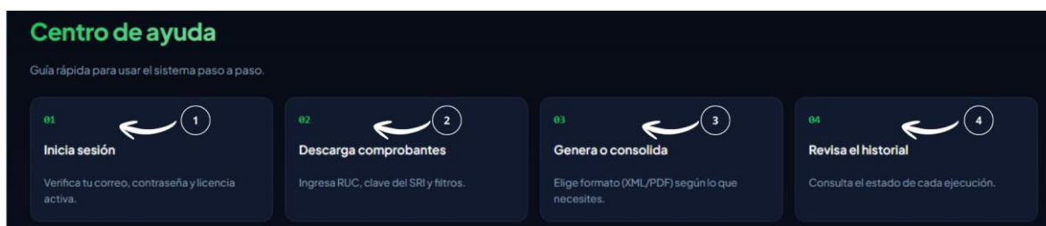
Figura 19. Quickstart cards
