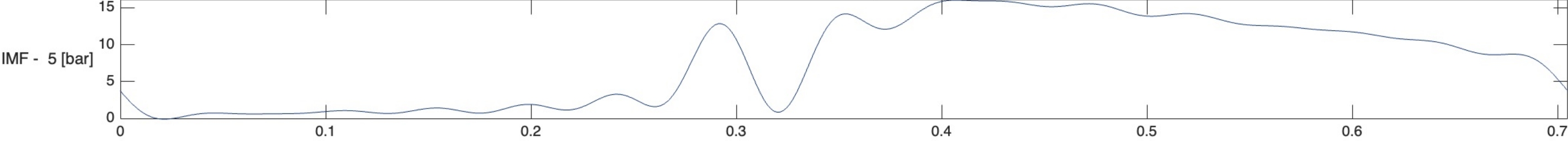
Original Signal
