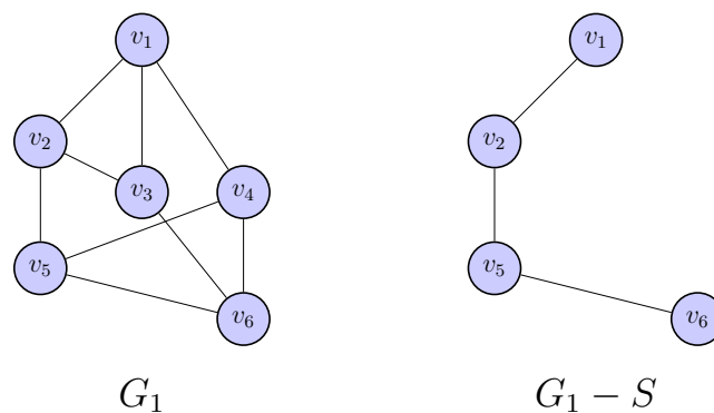
Figura 1.1.17: G_1 y G_1 - S
