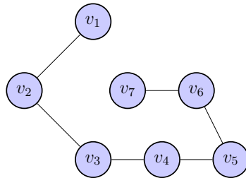
Figura 1.1.11: P^6 = v_1v_2v_3v_4v_5v_6v_7
