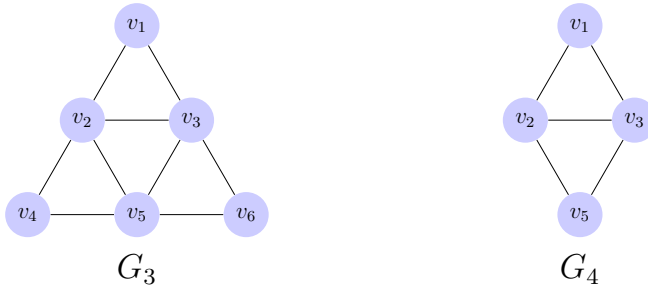
Figura 1.1.3: G_4 = G_3[W']
