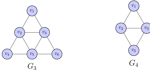
Figura 1.1.9: G_4 = G_3[W']
