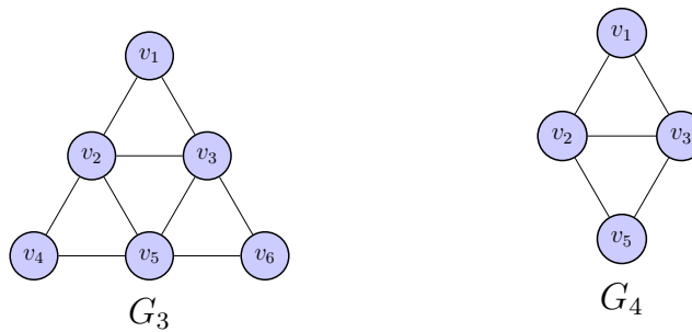
Figura 1.1.9: G_4 = G_3[W']
