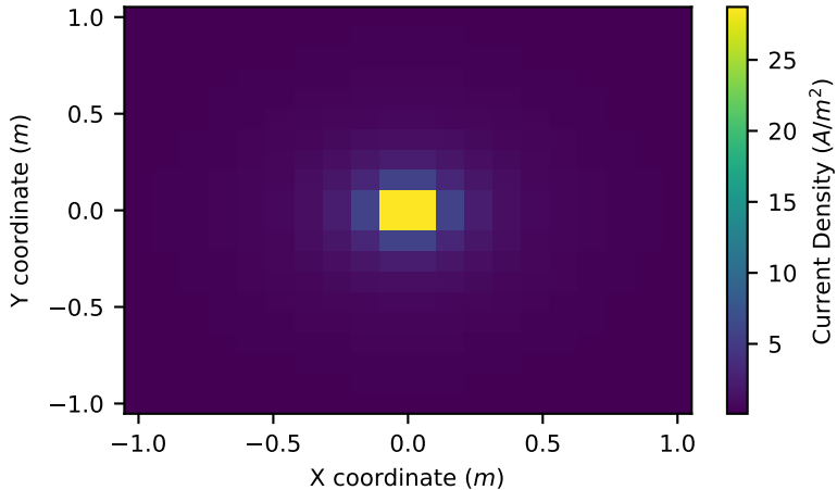
Current Density for a Point Current in a Halfspace
