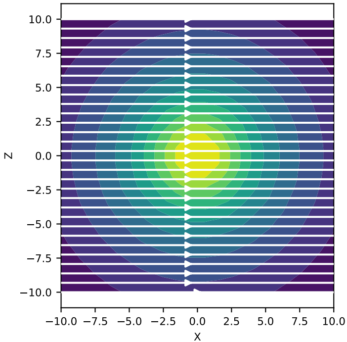
Vector potential at 1\text{e-}06 s
