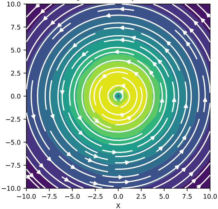
Magnetic flux density at 1\text{e-}06\text{ s}
