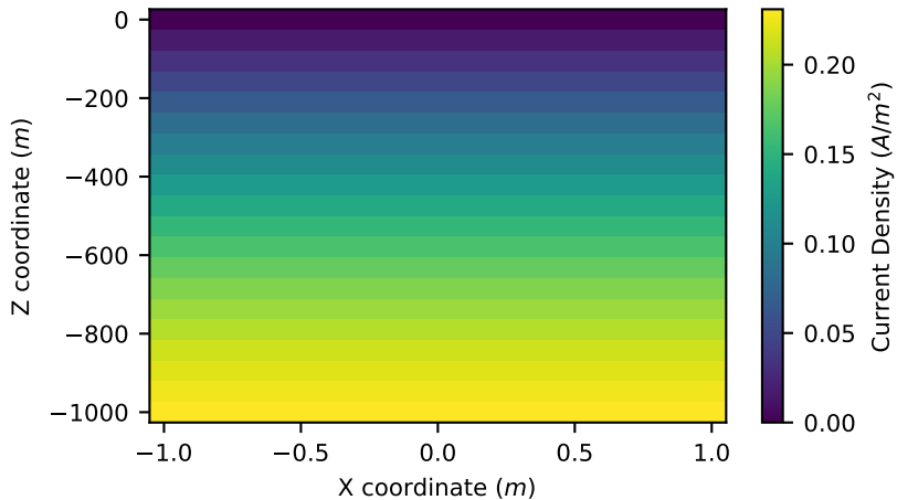
Current Density of a Transient Planewave in the x-direction in a Wholespace
