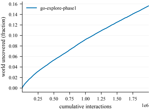
Cumulative coverage -- OpenFieldChamberCount10-610
