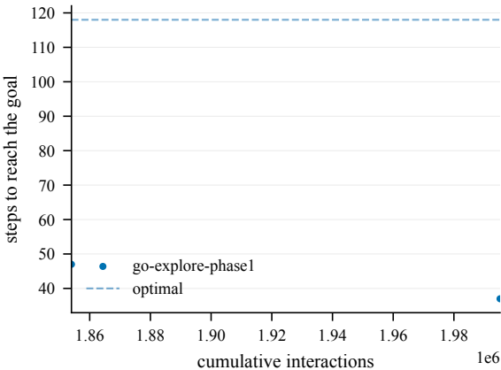
Steps to goal (train) -- OpenFieldChamberCount10-610
