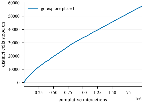
States discovered -- OpenFieldChamberCount10-610@2
