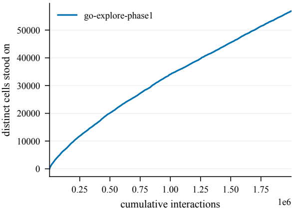
States discovered -- OpenFieldChamberCount10-610@4
