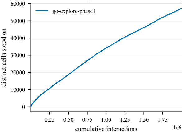
States discovered -- OpenFieldChamberCount4-500@1
