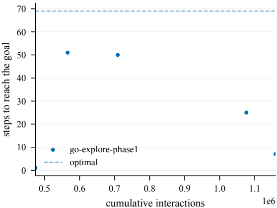
Steps to goal (train) -- OpenFieldChamberCount4-500@3
