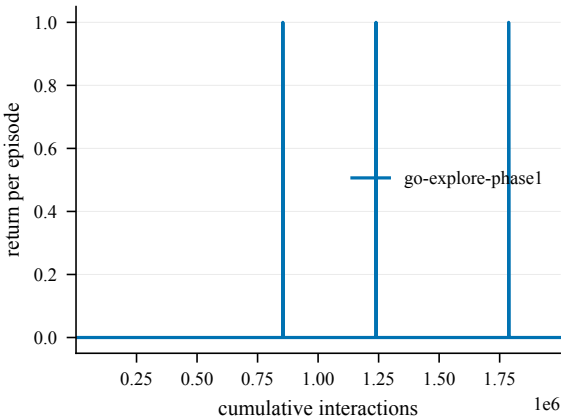
Return -- OpenFieldChamberCount6-530
