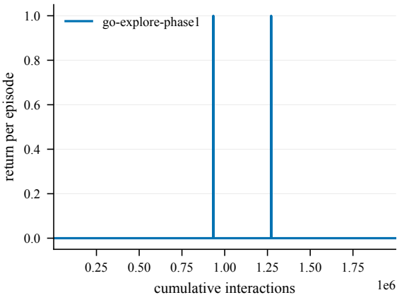
Return -- OpenFieldChamberCount6-530@3
