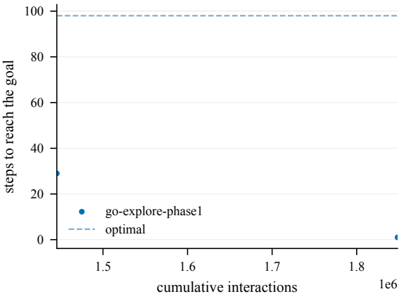
Steps to goal (train) -- OpenFieldChamberCount8-570
