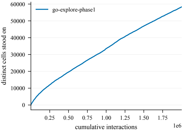
States discovered -- OpenFieldChamberCount8-570@1
