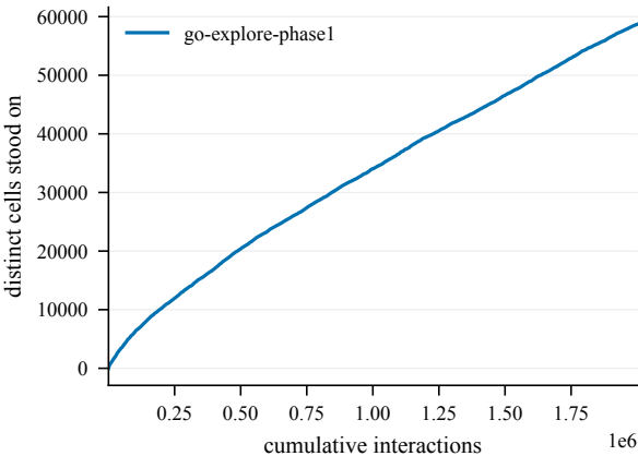
States discovered -- OpenFieldChamberCount8-570@3
