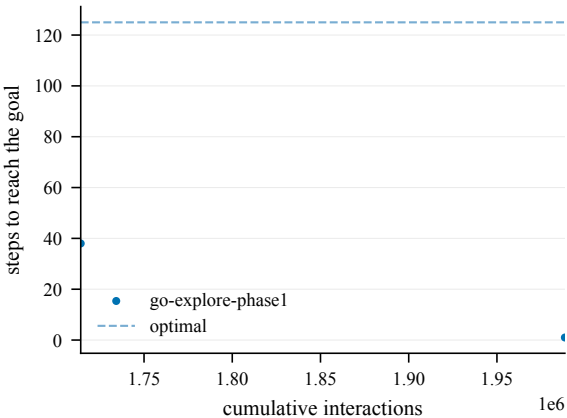
Steps to goal (train) -- OpenFieldChamberCount8-570@4
