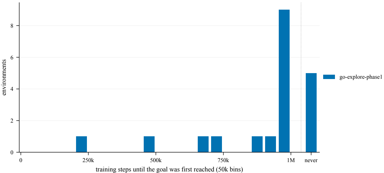
Steps to first goal, across the benchmark
