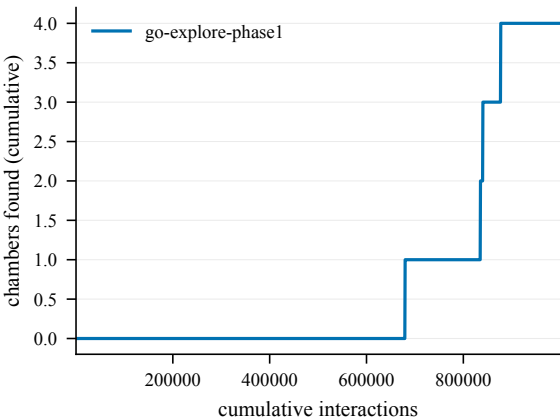
Chambers -- EnlargedChamberCount10-180@1
