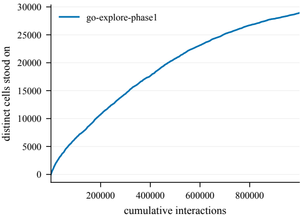
States discovered -- EnlargedChamberCount10-180@3
