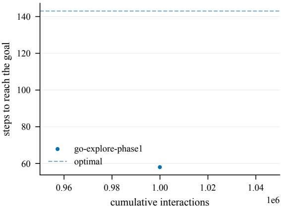
Steps to goal (train) -- EnlargedChamberCount10-180@4
