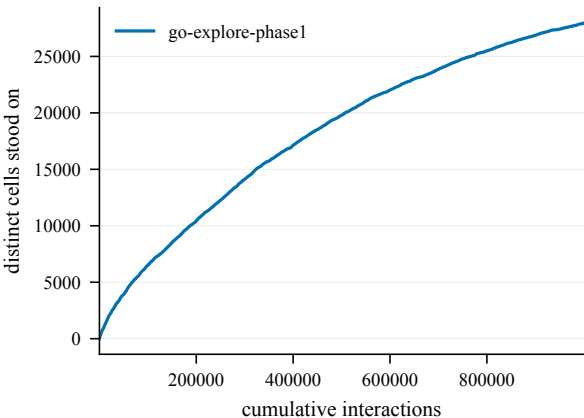
States discovered -- EnlargedChamberCount10-180@4
