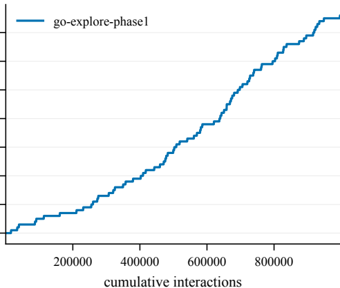
Goal reached -- EnlargedChamberCount2-60
