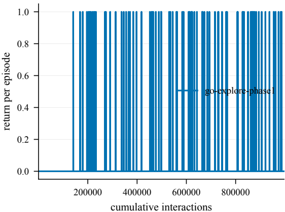
Return -- EnlargedChamberCount2-60@1
