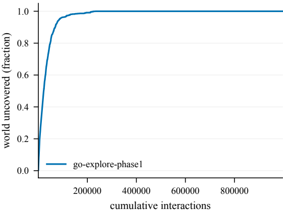
Cumulative coverage -- EnlargedChamberCount2-60@2
