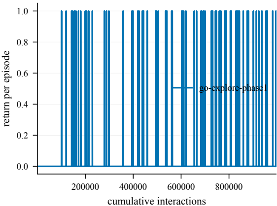
Return -- EnlargedChamberCount2-60@5
