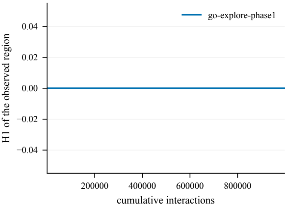
Discovered topology -- EnlargedChamberCount2-60@8
