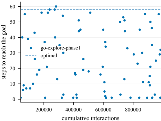
Steps to goal (train) -- EnlargedChamberCount2-60@9
