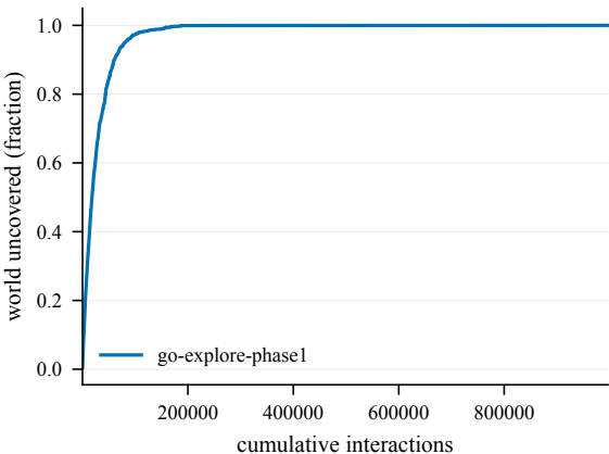
Cumulative coverage -- EnlargedChamberCount3-60@1
