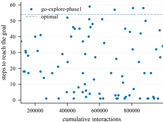
Steps to goal (train) -- EnlargedChamberCount3-60@4
