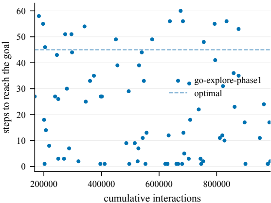
Steps to goal (train) -- EnlargedChamberCount3-60@7
