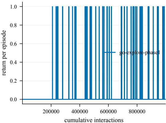
Return -- EnlargedChamberCount4-80@1
