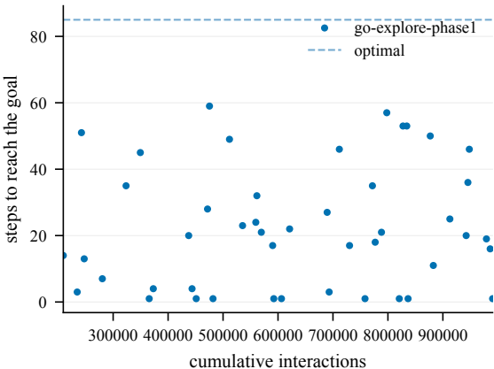
Steps to goal (train) -- EnlargedChamberCount4-80@1
