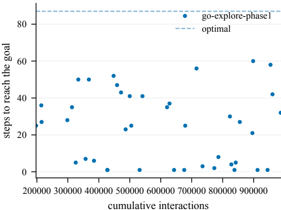
Steps to goal (train) -- EnlargedChamberCount4-80@6
