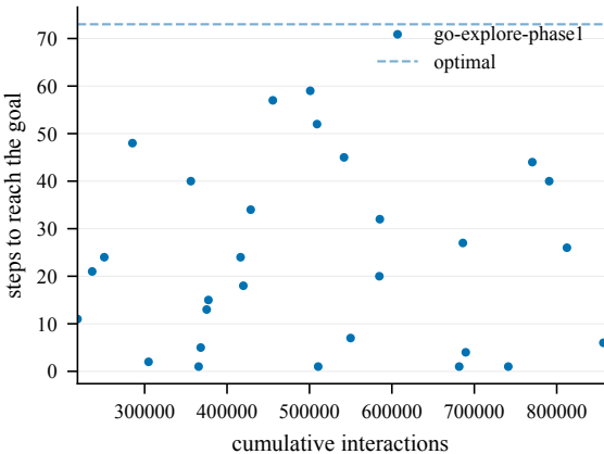
Steps to goal (train) -- EnlargedChamberCount4-80@9
