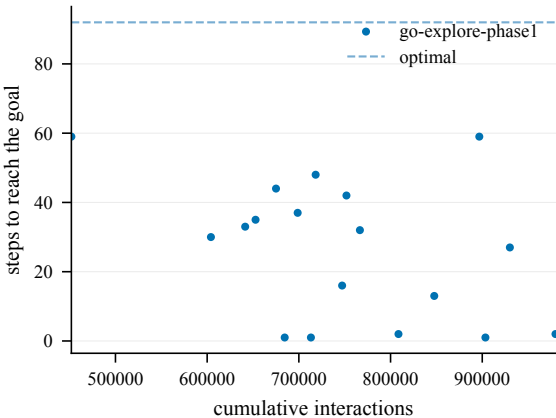
Steps to goal (train) -- EnlargedChamberCount5-100
