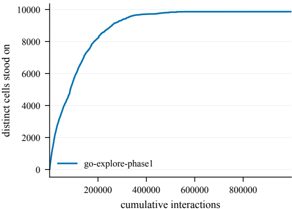
States discovered -- EnlargedChamberCount5-100
