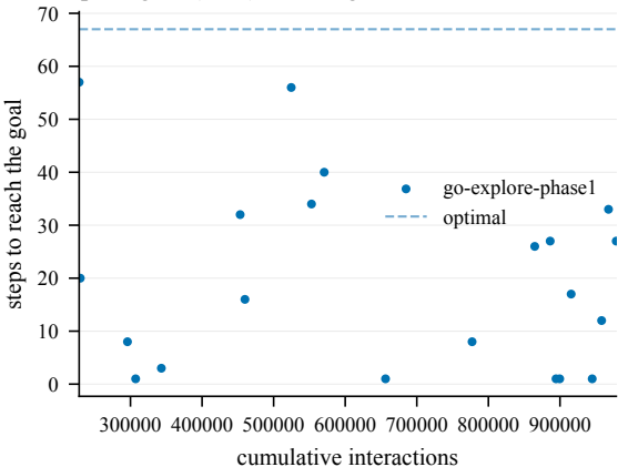
Steps to goal (train) -- EnlargedChamberCount5-100@1
