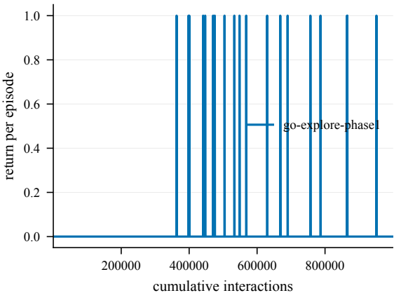
Return -- EnlargedChamberCount5-100@3
