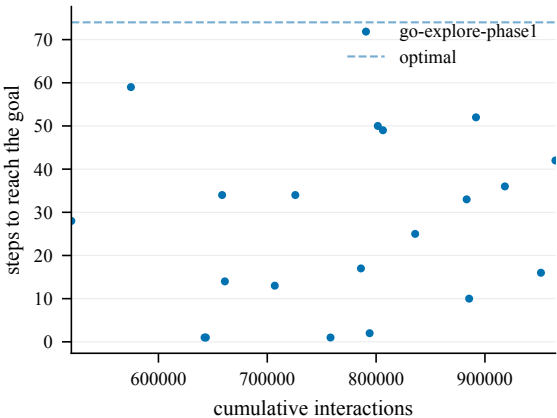
Steps to goal (train) -- EnlargedChamberCount5-100@4
